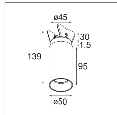
NYTO SEMI-RECESSED ADJUSTABLE 50
