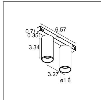
Nyto Track 48V Adjustable 1.6 2x
