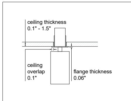
Flange Information
