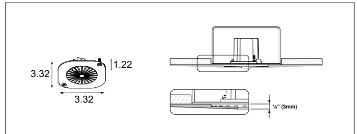
Recessed Trimless 0.4 1x DE (for installation with 4"x4" octagonal junction box)
