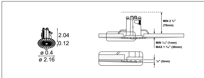
Recessed Trimless 0.4 1x DE (for installation without junction box)
