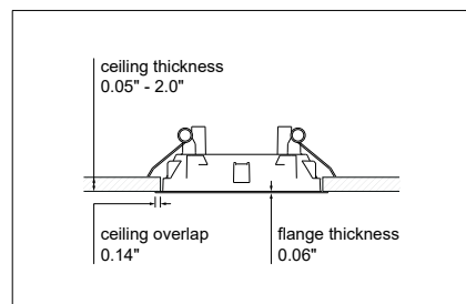
Deep Recessed 3.5 2x DE - Flange Information
