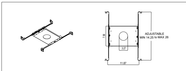
New Construction Frame for Modujack Round Deep Recessed 3.5 1x DE
