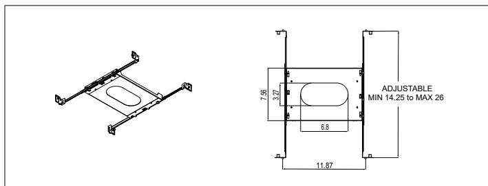
New Construction Frame for Modujack Round Deep Recessed 3.5 2x DE
