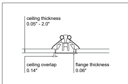
Deep Recessed 3.5 1x DE - Flange Information
