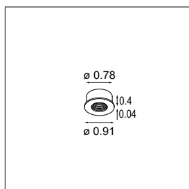
Stick Fixation Ring
