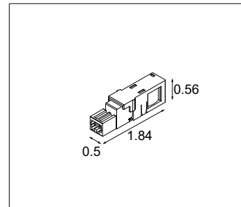
Male Connector
