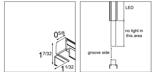
Linear Flaps
