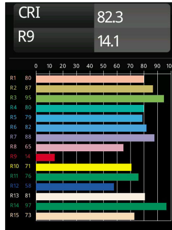
Pista Linear Nightlight Track 48V (values for 3000K)
