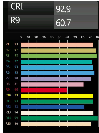
Pista Linear Light Track 48V (values for 3000K)
