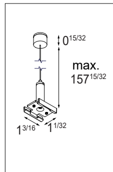
Suspension Cable
