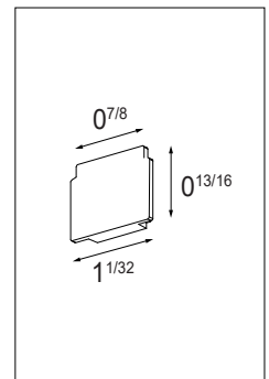
Surface Endplates
