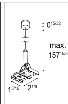
Twin Suspension Cable
