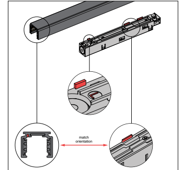
Power feed left - Groove orientation
