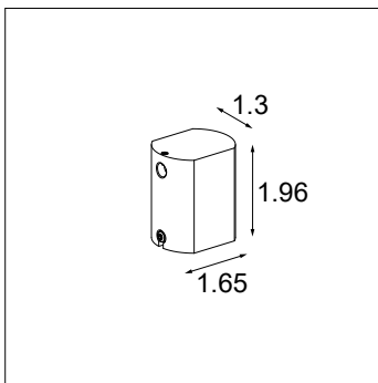
Connection Box for installation without junction box
