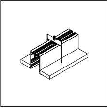
93560057 SLD50 RECESSED BRACKET
