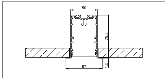
SLD50 POLY IN
