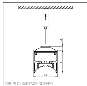
DRUPL70 SURFACE CURVED
