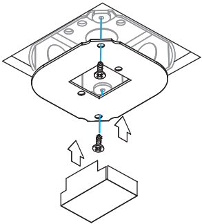
FOR OCTAGONAL BOX 4" by 4" (POUR OCTAGONAL BOX 4 "par 4")
